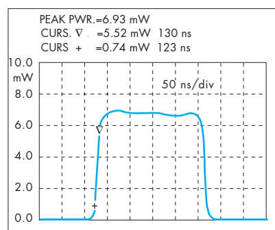
Fig. 14: Screen display of envelope power
