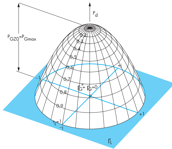
Fig. 9: Net power of a source, plotted versus the plane of the complex load reflection coefficient \Gamma_L . The grid lines of the 3-D surface are obtained by projection of the circles r_\Gamma = \text{const.} and the straight lines \Phi_\Gamma = \text{const.}
