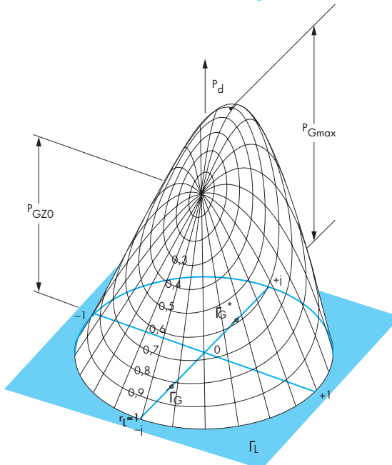
c) mismatched source, r_G = 0.5 (SWR = 3; \Phi_G = -90^\circ )
