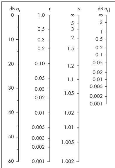
Fig. 6 Nomogram for reflection coefficient r , SWR, return loss \alpha , and mismatch loss \alpha_d
