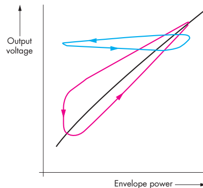
Fig. 31: Dynamic transfer characteristic of a diode sensor outside the square-law region with low-frequency (red) and high-frequency (blue) amplitude modulation (static characteristic in black)
