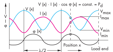
Fig. 11: Voltage and current on a line with mismatched load ( r_L = 0.5 ; \Phi_L = 0^\circ ); \lambda = line wavelength, \varphi = phase shift between V and I
