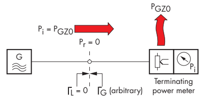
Fig. 8: Measurement of source power delivered to Z_0 load
