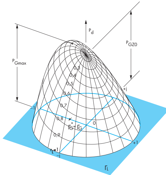
b) mismatched source, r_G = 0.3 (SWR = 2; \Phi_G = 180^\circ )
