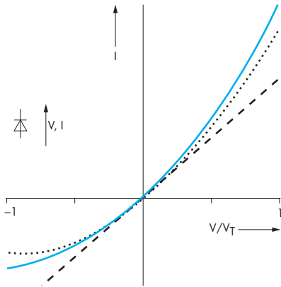
Fig. 26: Current-voltage characteristic of a Schottky diode in the square-law region (blue); dotted: square approximation; dashed: I = V/R_0 , where R_0 is the video impedance without external bias; V_T = temperature voltage (25 to 35 mV)
