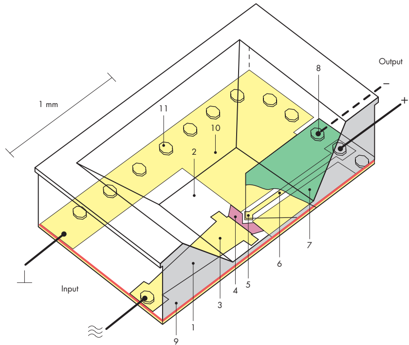
Fig. 20: Sectional view of measurement cell:
